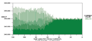
Adaptive control is a unique but standard feature that keeps your "package" accurately tuned to your process, without shutting down the loop.
