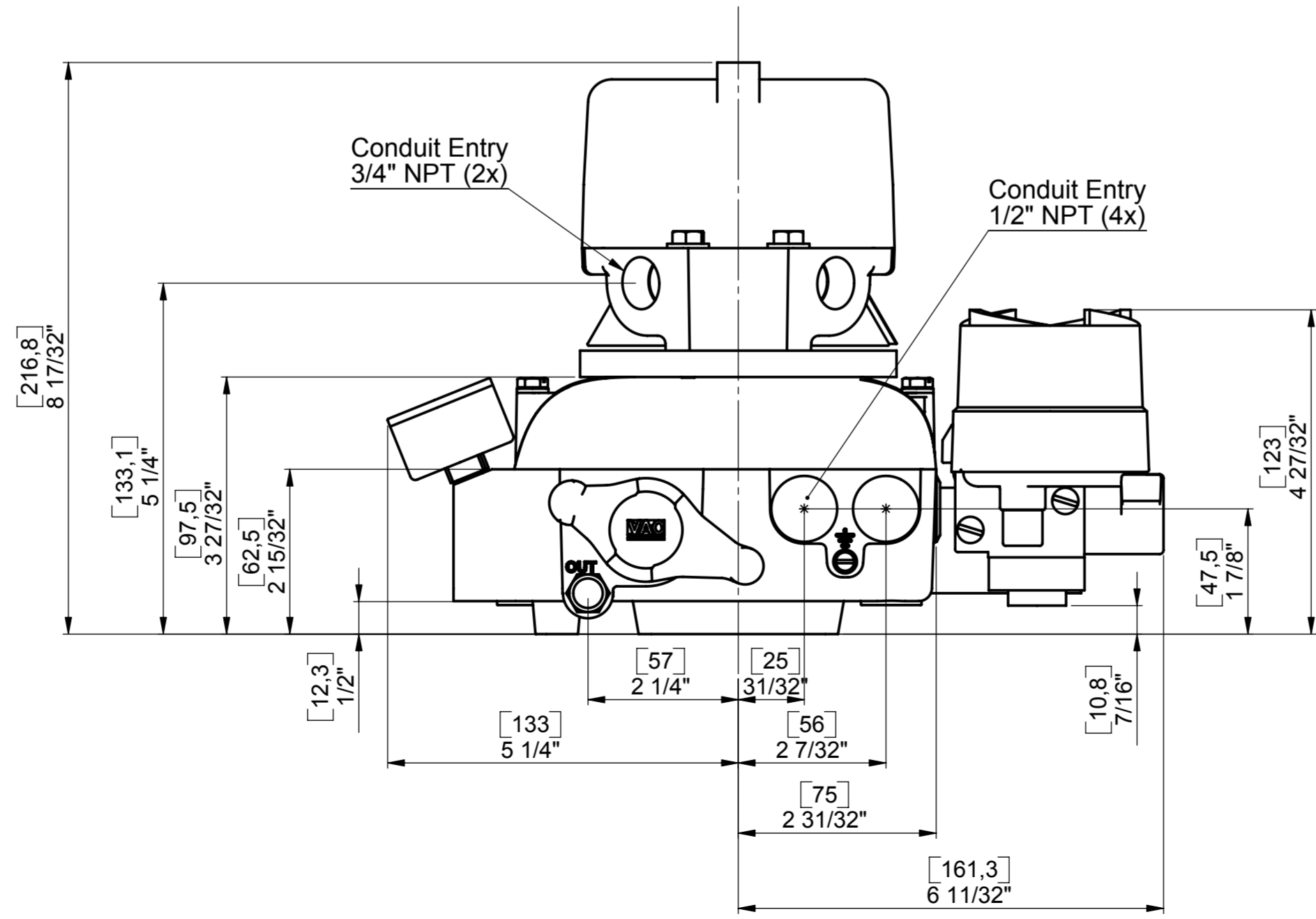
Dimensional Drawing VAC Positioner V200 EX Stonel Quartz + ABB Exd
